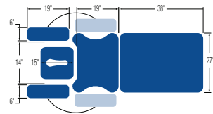
3 piece head section
