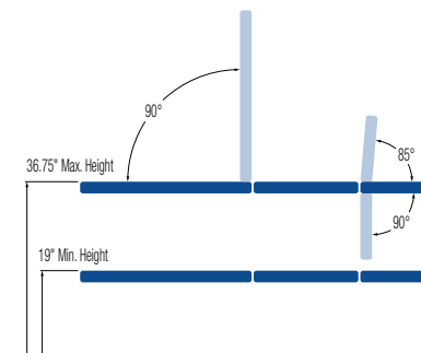
Optional rear leg soft touch footswitch configuration
