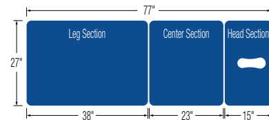
Standard Model
