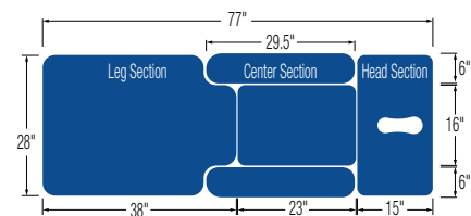
Center Section with Collapsible Sides
