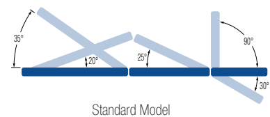
Standard Model
