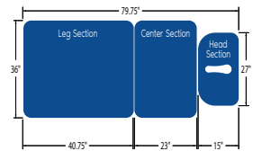
Standard Model
