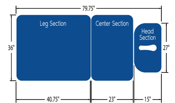
Standard Model
