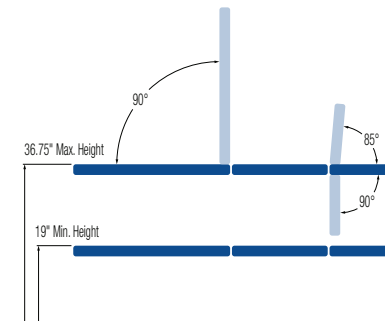
Optional rear leg soft touch footswitch configuration
