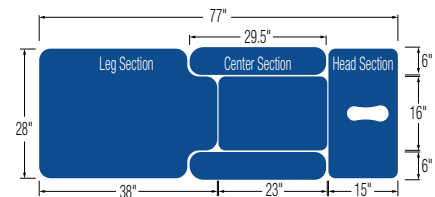
Center Section with Collapsible Sides
