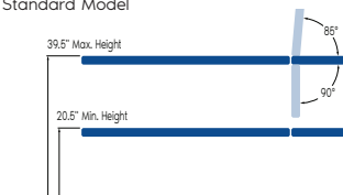
Standard Model
